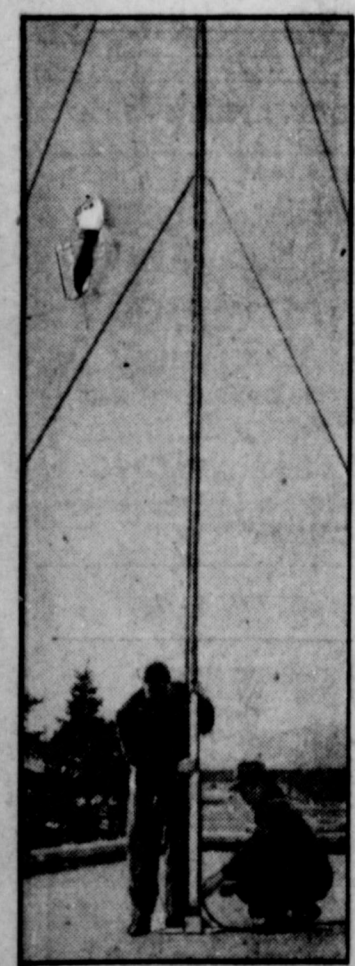
"CAN U READ ME?"—Police radio operators Thomas F. Korn, left, and Orville Wingate inspect their 30-foot-high, 500-watt beer can transmission antenna in Chicago, Ill. The 77 cans, welded together, tower right out of the picture. Base insulator is a quart ginger ale bottle, which rests in a coffee can. Guy wires are fashioned of plastic clothesline.
