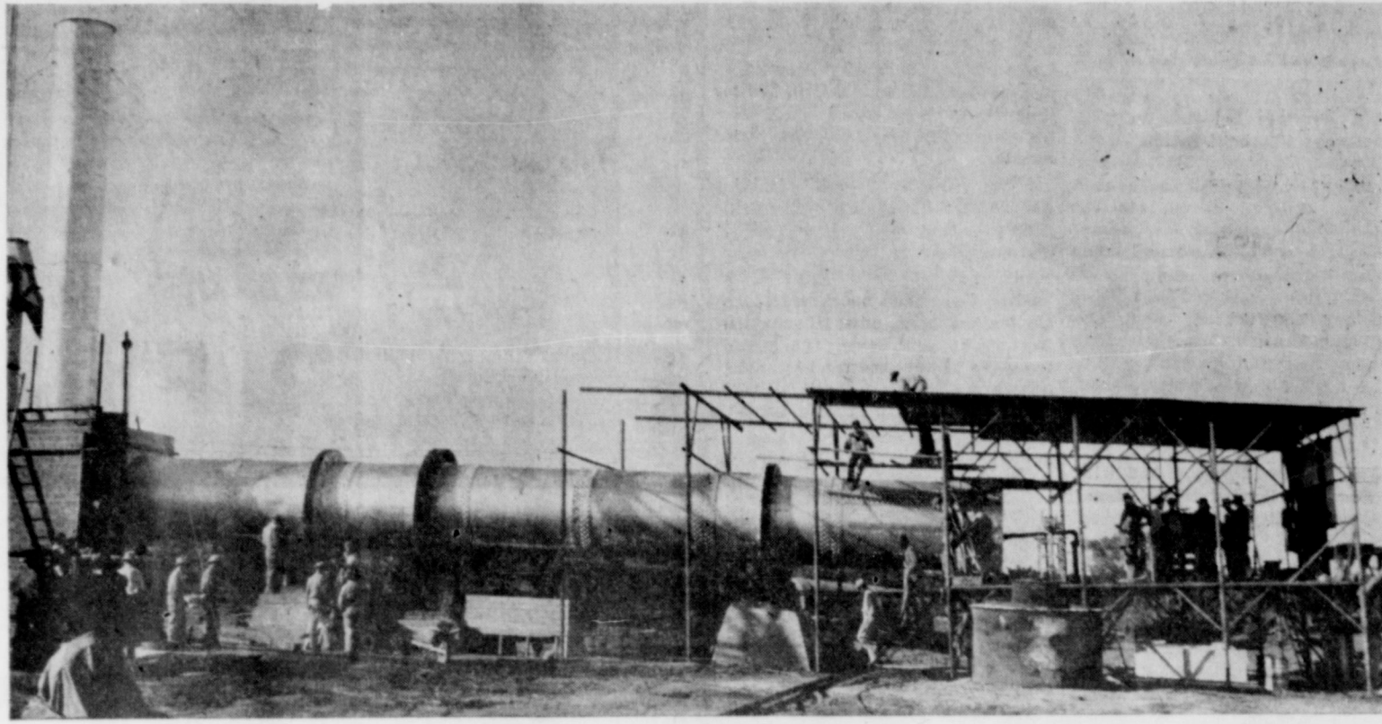
This was the way it looked when the first big kiln of the Texas Lightweight Aggregate Company in Eastland began turning out Haydite for the first time recently. In the picture are workmen at the plant and a number of Eastland businessmen who were on hand for the start of operations. Raw clay from the hillside at left of picture enters a mixing device shown at extreme left, is injected into the kiln and undergoes a sort of explosive action that fills it with tiny air bubbles, and then tumbles down the kiln as it is baked. The kiln slowly revolves. (Photo by Shultz)
