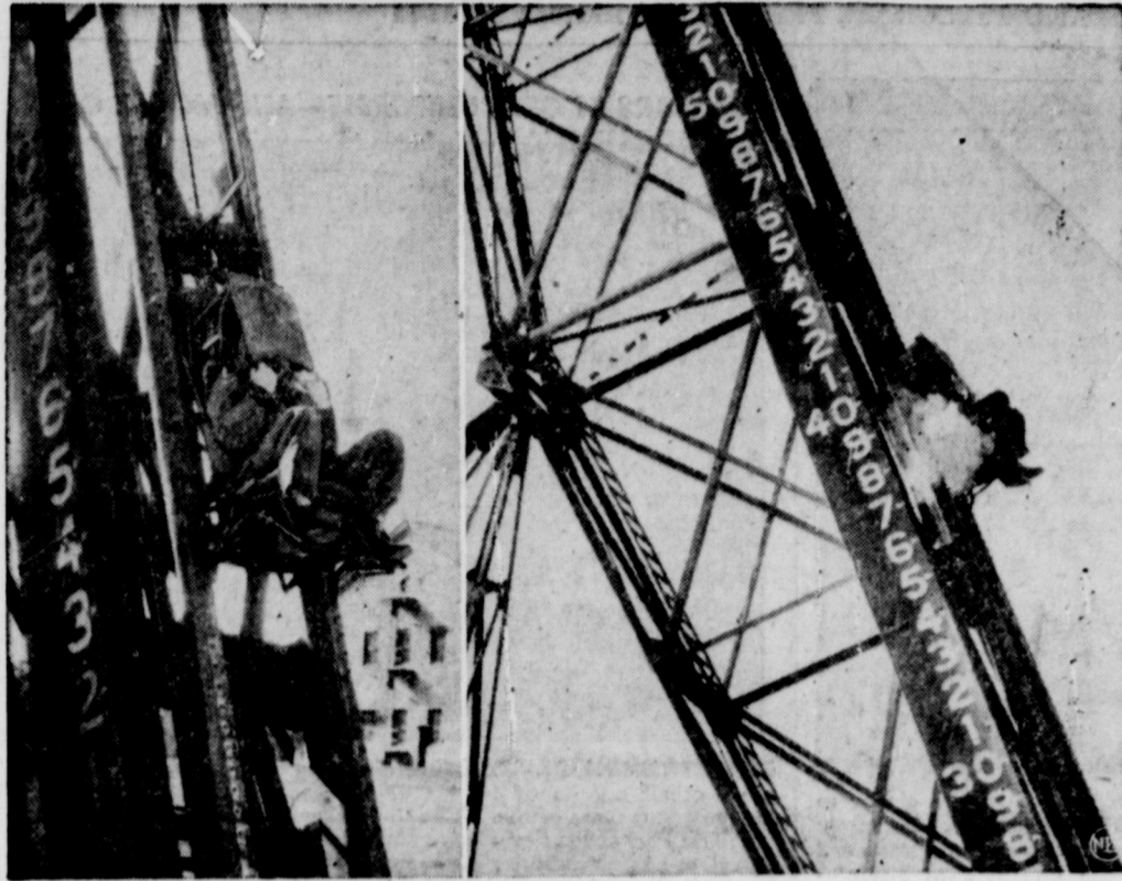
"HOT, DRY RUN" FOR JET "SCRAM SEAT"—Zoom! To the top of a 105-foot tower in two seconds shoots Marine Sgt. Thomas W. Watson of Farmville, Va. At the Philadelphia Naval Base, Watson was testing a skyrocket device which duplicates the "ride" of a jet pilot when he uses an automatic ejection seat to free himself from a crippled plane. The high speed of the seat started it smoking at 40 feet, right, but the sergeant was unharmed. The skyrocket trainer will be used to teach pilots what to expect when they spring out of a crippled jet and parachute to earth.
