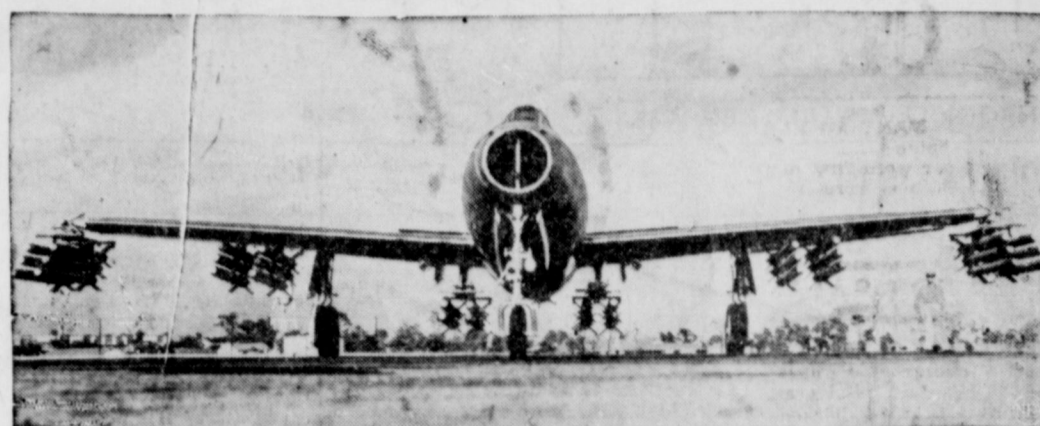
PACKED WITH POWER—Loaded like a fireworks factory, the new Republic F-84-E Thunderjet, high-speed, long-range fighter prepares to go into action in air-ground maneuvers at Elgin Air Force Base, Fla. The 600-mile-per-hour plane—the Air Force's first jet propelled fighter bomber—carries clusters of 32 five-inch high-velocity aircraft rockets, giving it unprecedented power. Its fixed armament consists of six .50-caliber machine guns.
