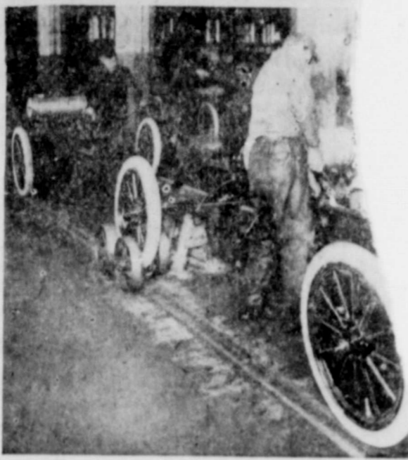
This is mass production—1913 style! The moving assembly introduced by Henry Ford that spring. In August, the first One month later, when this photo was taken at Ford Model T assembly time had been cut from 14 hours to 93 min.
