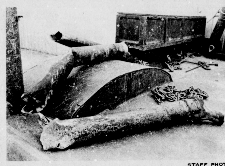
STAFF PHOTO SCHOOL BUS DRIVE SHAFT — The drive shaft of a Lockney school bus lies in three pieces on a wrecker. The drive shaft broke as the bus, with the junior varsity football team aboard, was enroute to Idalou Thursday afternoon.
