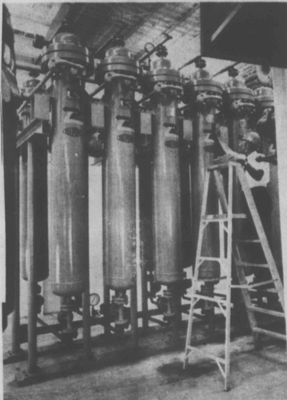
DESALTING PLANT AT PLAINS--100,000 gallons of good quality water per day are produced by "Permasep" permeators in Plains, Texas, plant. Dissolved solids are removed from brackish well water before it is placed in the city distribution system.
