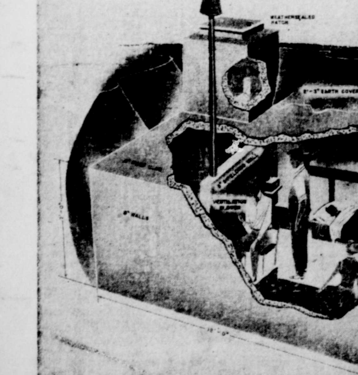
FALLOUT SHELTER for a family of four to six shows how a layer of 2 feet 3 inches of earth over a 6-inch concrete roof slab offers good protection even to highly radioactive fallout zones. Cost of this backyard shelter would range from $1,000 to $1,500, including ventilation equipment. It is recommended by the Office of Civil and Defense Mobilization as the best family fallout shelter for a moderate price, but other less expensive basement designs are available. Further details appear in Technical Bulletin TB-53 issued by OCDM headquarters at Battle Creek, Michigan. (OCDM Photos)
