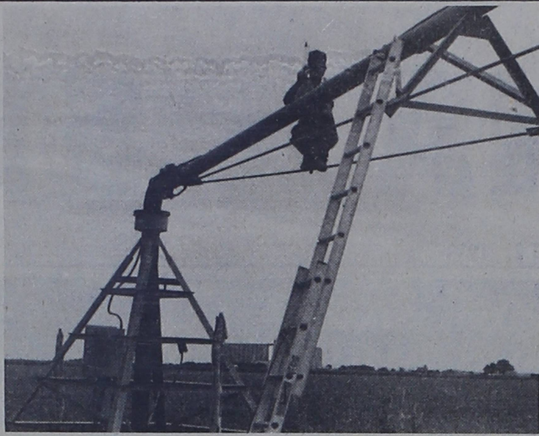
WATER FLOW CHECKED.... During a center-pivot sprinkler evaluation the water flow into the system is checked with a velocity meter. Henry Skala, SCS employee, is shown reading the Cox velocity meter.
