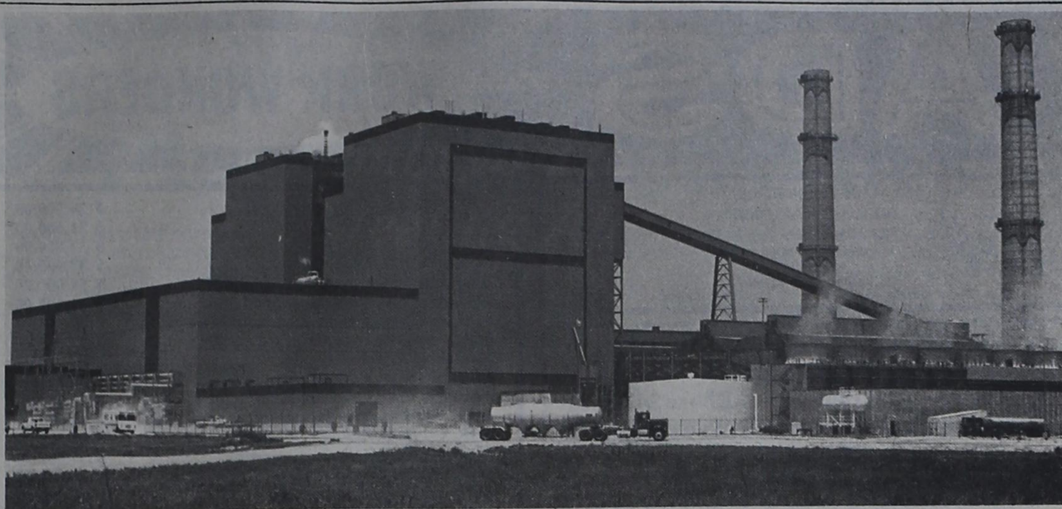
TOLK STATION...SPS' Tolk Station Units No. 1 and No. 2, near Muleshoe, Texas, both are producing electricity now. Wyoming coal is burned in steam boilers in the 20-stories-tall boilerhouses, center. Then steam flow drives each of the 561,000-kilowatt turbine-generators, which produce the electricity. The boiler flue gasses are cleaned in baghouses before exiting 400-foot stacks, right. (SPS Photo)
