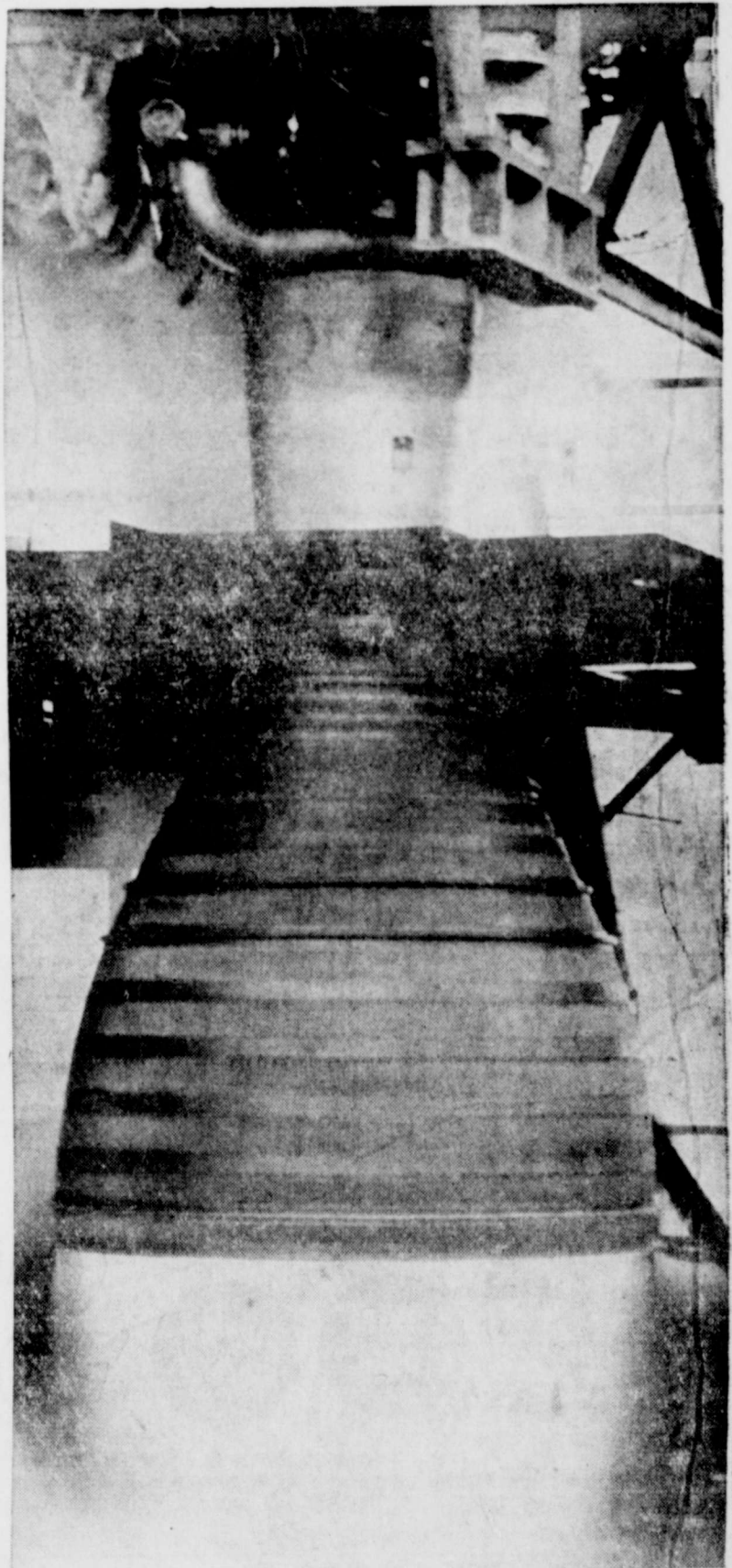
FIRST PHOTOGRAPH released of the Rocketdyne 400,000 lbs. thrust class research and development liquid propellant rocket engine being test fired at Propulsion Field Laboratory in Santa Susana Mountains, California. It was developed by Rocketdyne, a Division of North American Aviation, Inc., under a contract with the U. S. Air Force. The engine is contributing information on combustion, turbo machinery design and systems operation for very high thrust engine. At the present time this Rocketdyne engine is not scheduled for any specific vehicle. Technical direction of program is being administered by Air Force by Rocket Propulsion Development Division, Edwards Air Force Base.
