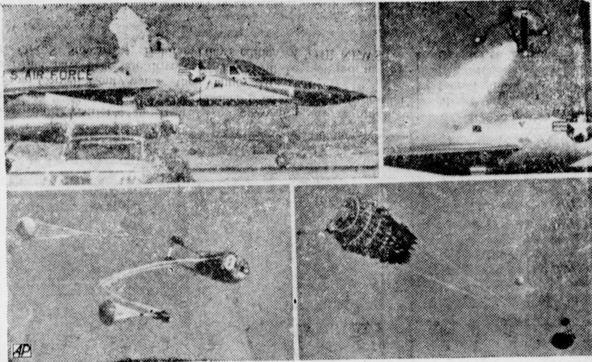
EJECTION BY ROCKET—An escape capsule powered by rockets breaks through the top (upper left) of a B58 Hustler bomber during a test of the ejection system at Edwards Air Force Base, Calif. The capsule, with a dummy inside, zooms (right) toward an altitude of 250 feet where two parachutes (lower left) open for the descent. Main chute starts to lower the
