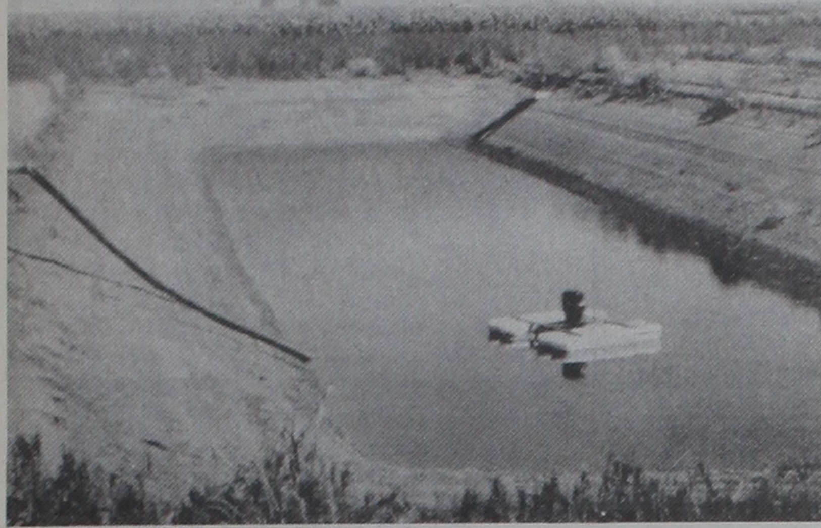
TAILWATER RETURN PIT....Many High Plains producers have constructed tailwater return pits to collect irrigation water that would otherwise be lost as tailwater. The collected water can then be pumped back onto the field for re-use.
