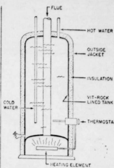
Cross-section view of a modern automatic water heater.
