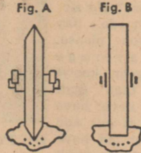
(A) Rolkleen packs soil completely around seeds, leaves moisture-catching mulch behind in its track. (B) Flat press wheel packs soil unevenly, makes a hard crust.
