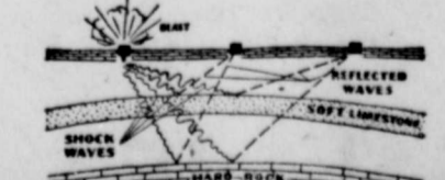
Sound waves from an explosion penetrate the earth, then rebound from various strata to indicate the structures most favorable for oil or gas.
