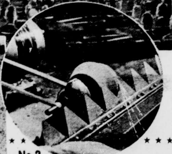
No. 2 See this quick, easy way to sharpen the knives of your mower.
