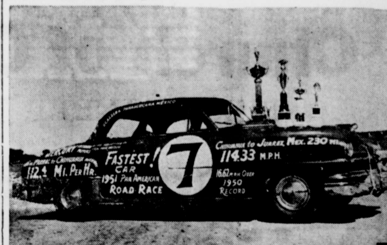
New lap record of 114.33 M.P.H. in Mexico race wins special award. This Tony Bettenhausen-Chrysler combination, running in the 1951 Mexican Road Race copped four of the automotive world's coveted trophies for engineering excellence. The Kiekhaefer (Mercury Outboard Motor) Corp., who entered the car, had its engineers switch their know-how from outboards to automotive engines in preparation for the South-of-the-Border grueling grind.
