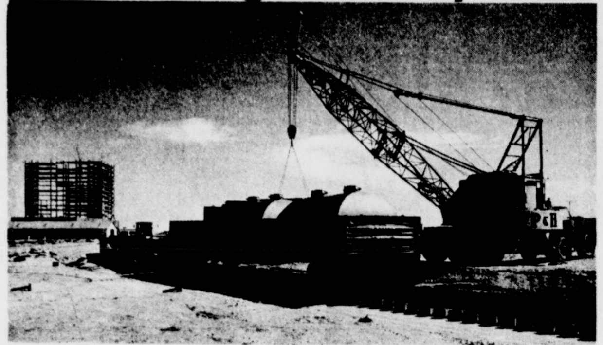
TOLK PLANT — Structural steel of Southwestern Public Service Company's new coal-fired Tolk Station stands in the background as equipment is unloaded from railroad cars inside the plant grounds.
