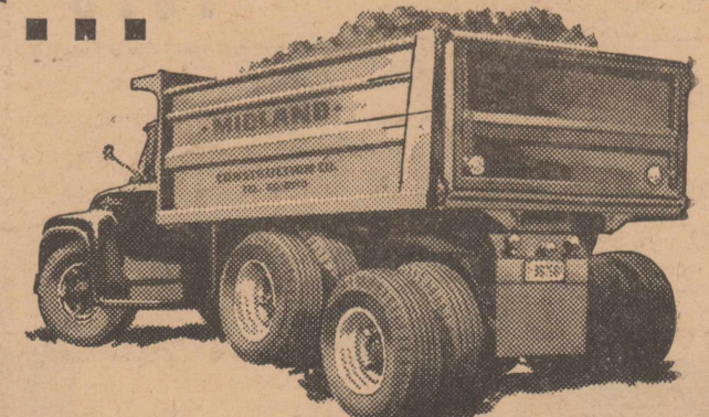
Factory-built tandem-axle T-800, 42,000 lbs. GVW, 65,000 lbs. GCW. Choice of two V-8's with up to 212 h.p.
