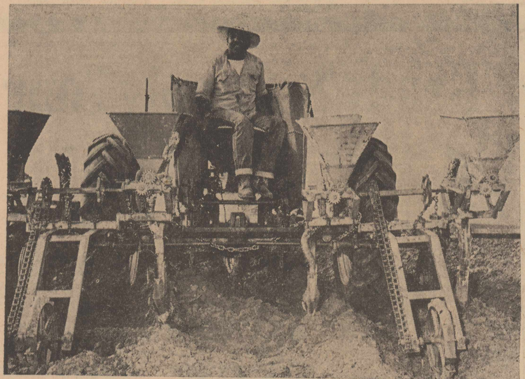
This Mexican laborer is applying Mathieson Ammo-Phos on the J. L. Snider farm at Circle. He is using a four-row John Blue distributor that J. L. attached to the tool bar of his tractor. The Ammo-Phos Plant Food is being put just below and beside the proposed seed bed for greatest availability, and the Ammo-Phos 11-48-0 is being applied at a rate of 125 lbs. per acre.
