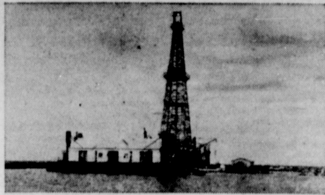
WORLD'S DEEPEST WELL —Prospects for oil production are encouraging at this record depth well which has "bottomed" at 22,559 feet. It was drilled by barge-mounted rig of Richardson & Bass in marsh country south of New Orleans, La. Drillers report that record depth was reached without a single drilling pipe failure. All the drill pipe and wire rope were supplied by Jones & Laughlin Steel Corporation. The "hole" is now being conditioned for oil production in zones above the deepest penetration. Previous record depth was 21,482 feet, set in Kern County, Calif.
