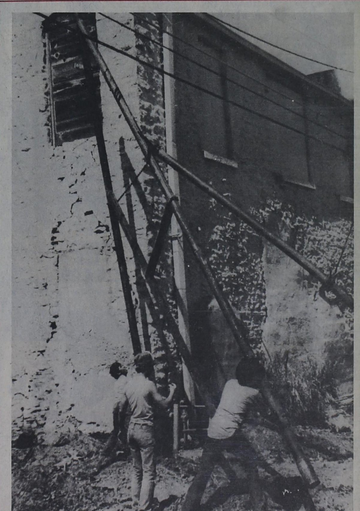
SHORING UP THE WALLS - Temporary support beams were installed this week on the south and west rear walls of the Algeria building downtown. The special support provides a safety measure while the Garza Heritage Association looks for funding to make more permanent repairs.
