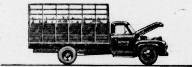
NOW 1 TON MORE GVW —Ford F-600 "2-tonner" has GVW boosted to 18,000 lbs. when equipped with heavy-duty rear axle, heavy-duty springs, 6-stud wheels, and 140-h.p. Short Stroke V-8 engine.
