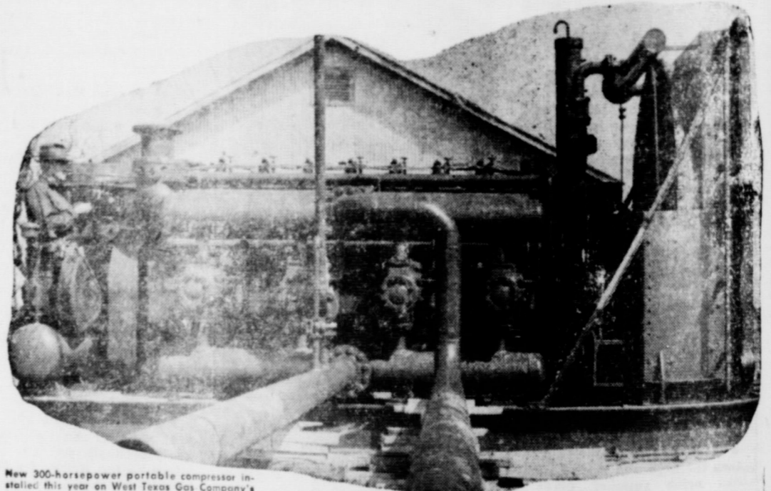
New 300-horsepower portable compressor installed this year on West Texas Gas Company's transmission line.
