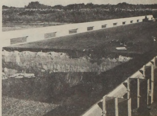
Gaping approach to Quitaque Creek bridge.
