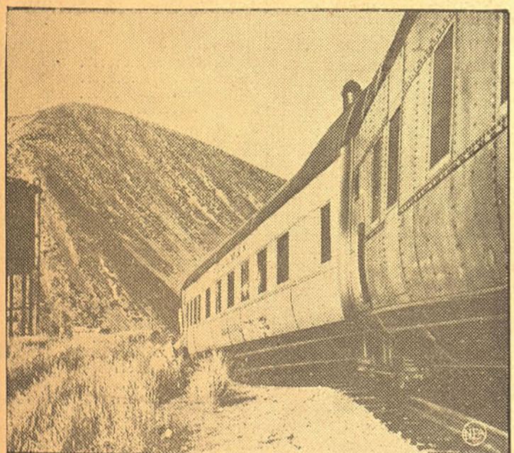
In one of the first accidents ever to befall a modern streamlined train, two cars of the "City of Portland," which makes the Chicago-Portland, Ore., run, longest in the nation, are shown above, twisted off the rails in a Wyoming canyon. After being derailed, the cars sped over the ties for a quarter mile. No one was injured.
